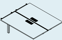
DT-AU Double Side Extension Table 双边增连台 W11000/1100/1200/1400/ 1500/1600/1800/2000/ 2200/2400 D1225/1425/1625 H745
